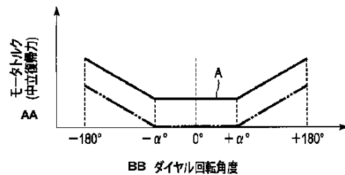
AA Motor torque (force to return to neutral) BB Dial rotation angle
