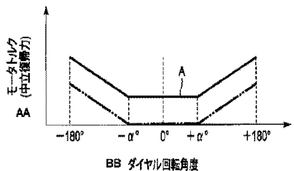
AA Motor torque (force to return to neutral) BB Dial rotation angle
